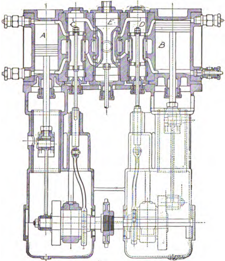
FIG. 268.—Section of the Stearns Compound Steam Carriage Engine. A is the high-pressure cylinder; B, the low-pressure cylinder; C and D, the steam valves operated by single eccentrics; E, the central control valve and chamber.
